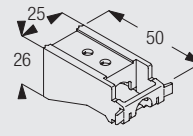
3655 Long universal bracket
